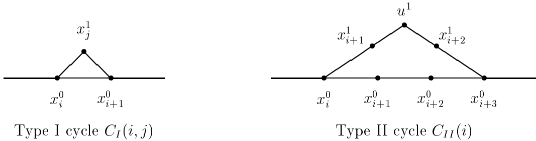
Figure 2: Two types of (n+1) -cycles.
