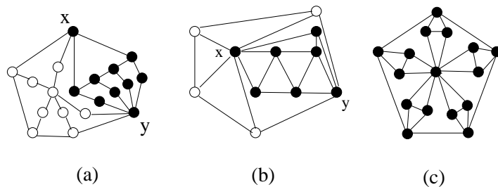
Figure 1: Planar graphs with circular chromatic numbers 3 and 4
